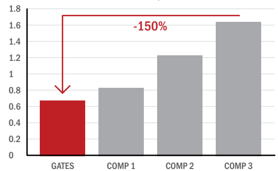
Force measured when minimum bend radius is achieved Measurement 1/4" size
